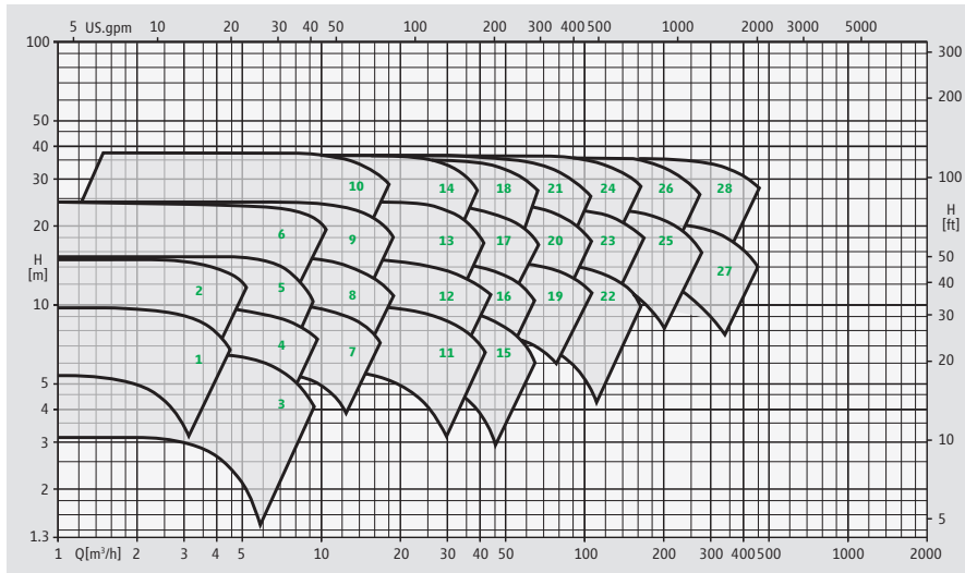
Characteristics diagram 1450 rpm 50 Hz
