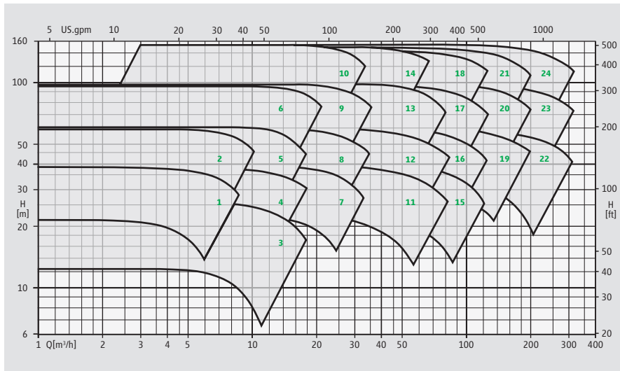
Characteristics diagram 2900 rpm 50 Hz
